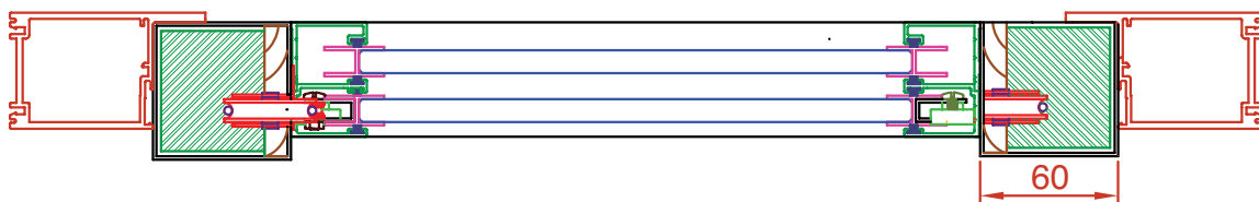
Section AA
