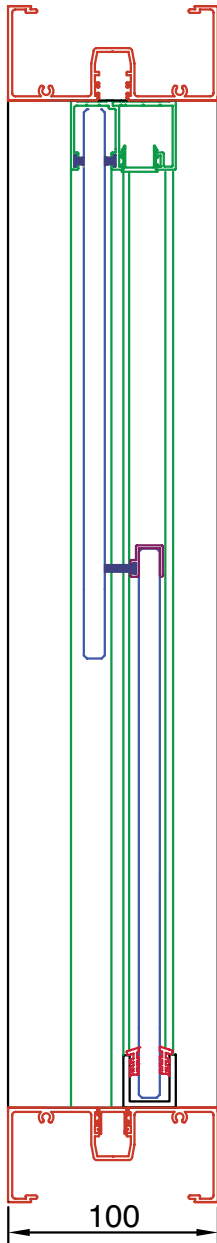
Section BB
