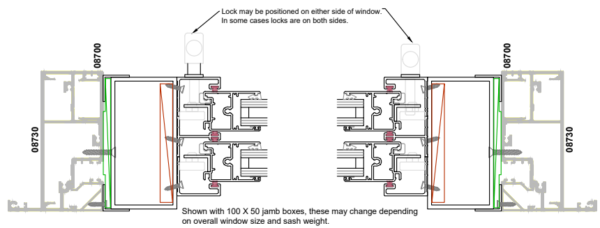
Section B:B
