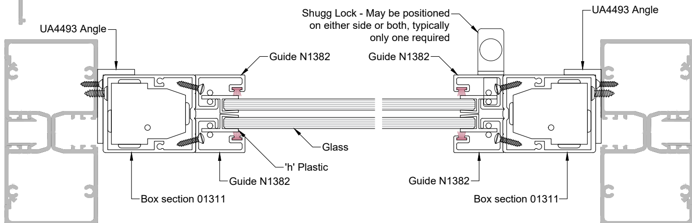
SECTION B-B
