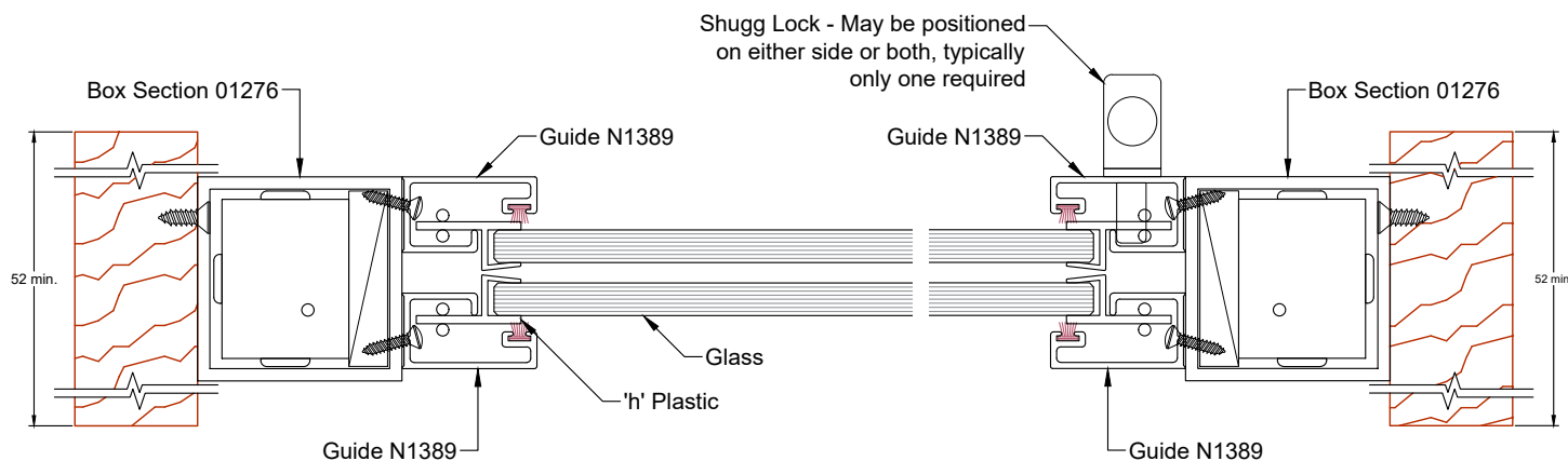
SECTION B-B
