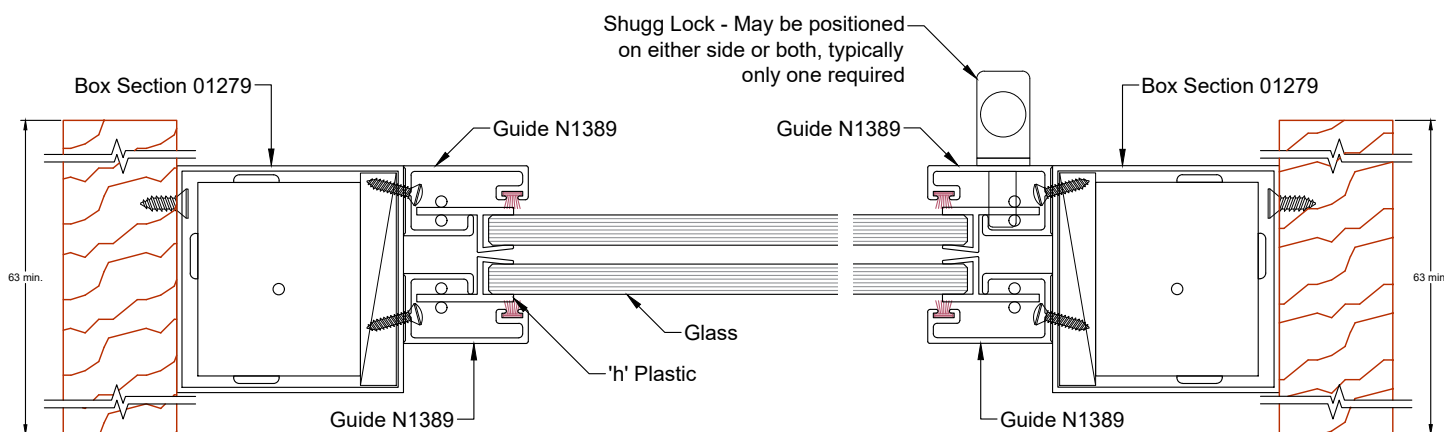
SECTION B-B
